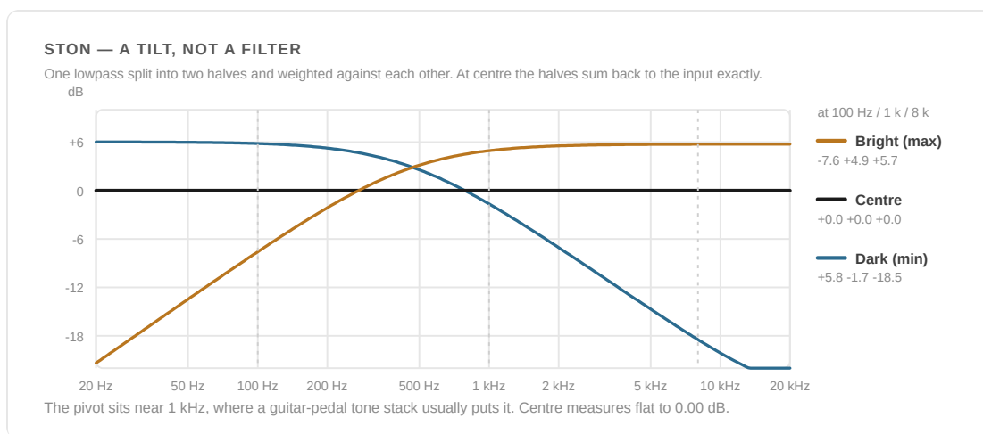
Figure 6.3 — The tilt, computed from the shipped one-pole. The three measured points quoted in the table above are marked; centre is a true bypass, which is the whole point of the topology.
