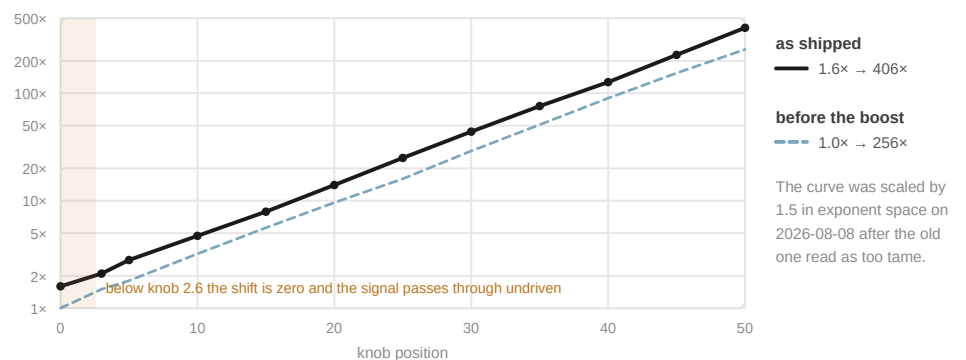
Figure 6.2 — Pre-gain into the clipper, on a log scale, so a straight line is a constant ratio per knob step. The dashed line is the taper as it shipped before 2026-08-08, kept here because the two are easy to confuse in older notes.
