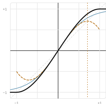
Figure 6.1 — The curve, and the two it was chosen over. The near-identical 1.5x - x^3 is the reason the coefficient matters: it folds back above x = 0.707 and would have made this a second wavfolder.
