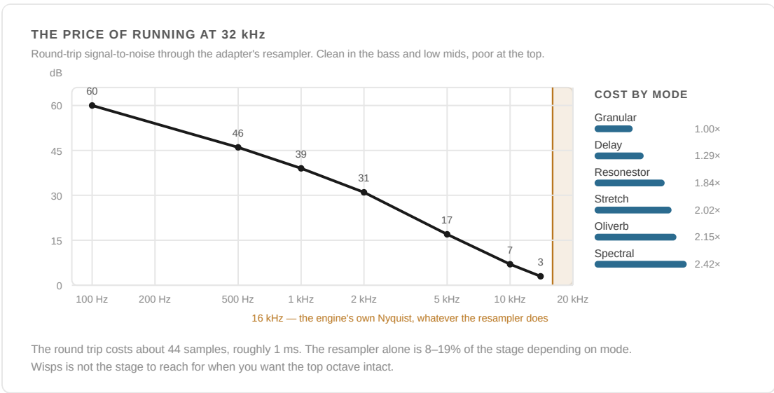
Figure 4.2 — Two costs in one picture: what the resampler does to the top of the band, and what each mode costs relative to Granular. Mode choice matters more than anything else here.
