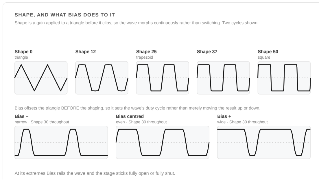
Figure 5.3 — Shape and Bias, computed through the shipped shaping code. Bias is added to the triangle before the shaping gain, which is why it sets the duty cycle rather than just offsetting the result.
