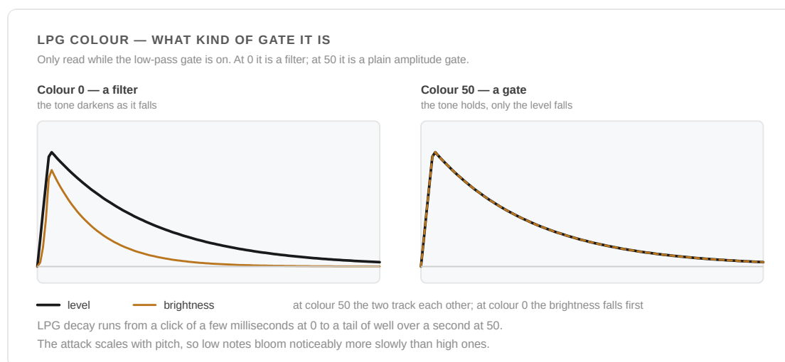
Figure 3.2 — LPG colour, at both ends of its travel. At 0 the brightness falls faster than the level — the vactrol behaviour; at 50 the two fall together and the tone holds.
