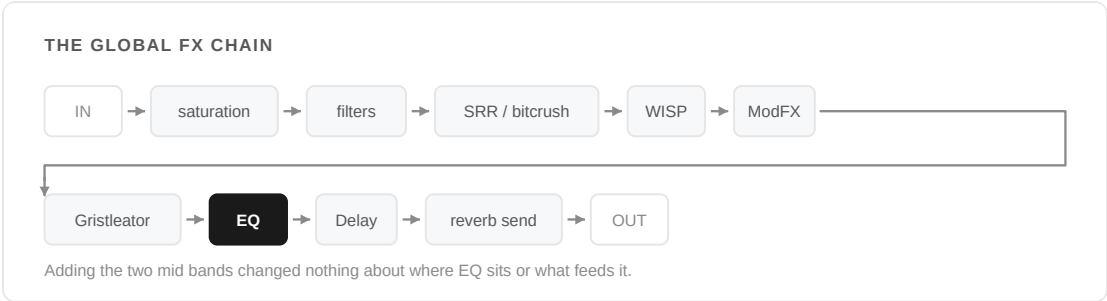
Figure 2.2 — The EQ occupies the same slot stock Deluge EQ always has, late in the global FX chain.
