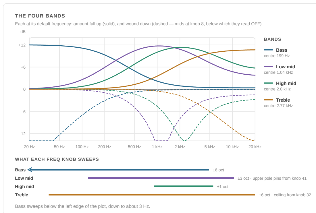
Figure 2.3 — Plotted from the same fixed-point law the audio path runs, so every centre frequency and every gain here is the number the menu reports. Note how much deeper a cut goes than a boost: that asymmetry is the amount law, not the plot.
