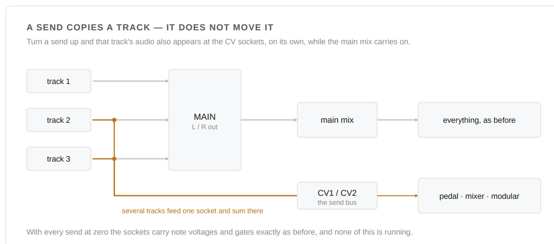
Figure 8.1 — A send copies a track to the sockets without taking it out of the main mix. Several tracks can feed one socket, and they sum there.
