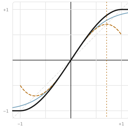
Figure 6.1 — The curve, and the two it was chosen over. The near-identical 1.5x - x^3 is the reason the coefficient matters: it folds back above x = 0.707 and would have made this a second wavefolder.
