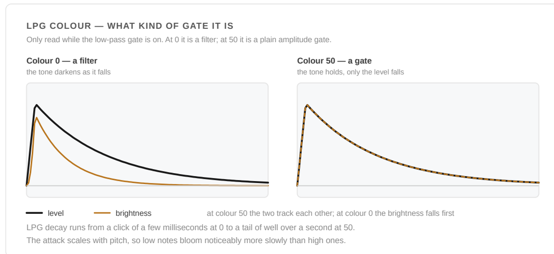
Figure 3.3 — LPG colour, at both ends of its travel. At 0 the brightness falls faster than the level — the vactrol behaviour; at 50 the two fall together and the tone holds.
