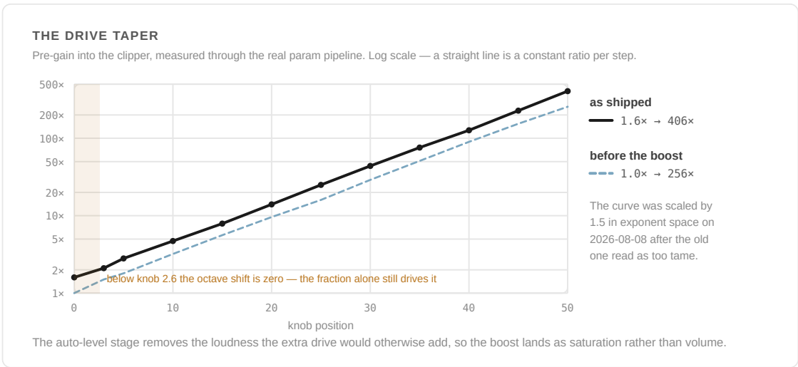
Figure 6.2 — Pre-gain into the clipper, on a log scale, so a straight line is a constant ratio per knob step. The dashed line is the taper as it shipped before 2026-08-08, kept here because the two are easy to confuse in older notes.
