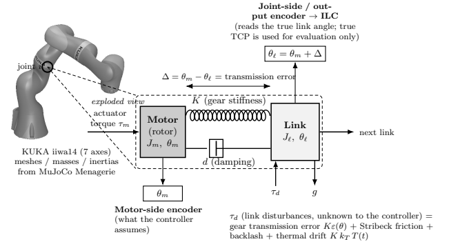
Figure 1: Flexible-joint drivetrain model. Every axis of the real iiwa14 is a two-mass system: a motor inertia J_m and a link inertia J_\ell joined by a torsional spring K and damper d . The controller plans on the rigid model ( \theta_\ell = \theta_m ); the link deflects, so \Delta = \theta_m - \theta_\ell is a real transmission error. The link also receives a disturbance torque \tau_d (transmission error, friction, backlash, thermal drift), unknown to the controller. The joint-side / output encoder reads the true link angle and feeds the ILC; the true Cartesian tool position is used only for evaluation.
