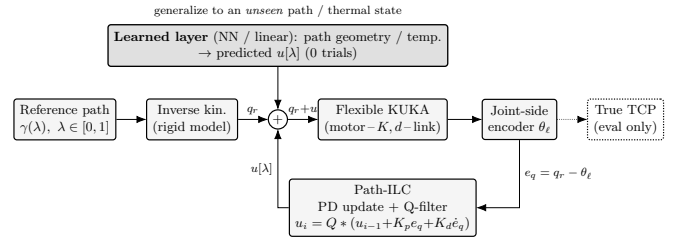
Figure 2: Control structure. The path-ILC learns u[\lambda] from the joint-side encoder error; the learned layer predicts u[\lambda] for an unseen path or thermal state with zero trials. The true TCP is used only for evaluation.
