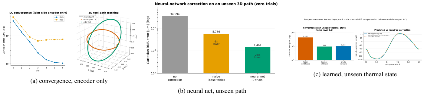
Figure 4: Headline results: (a) ILC convergence from the joint-side encoder only; (b) the neural-network layer on an unseen path, zero trials; (c) the temperature-aware learned layer at an unseen thermal state.
