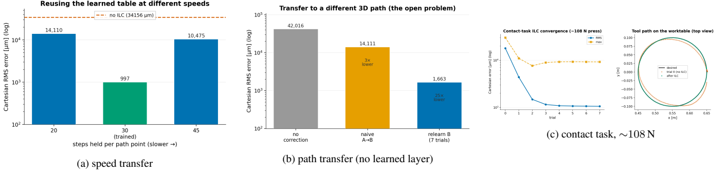
Figure 5: Further KUKA experiments: (a) reusing the table at other speeds; (b) path A→B transfer without the learned layer; (c) ILC on a tool pressed on a worktable.
