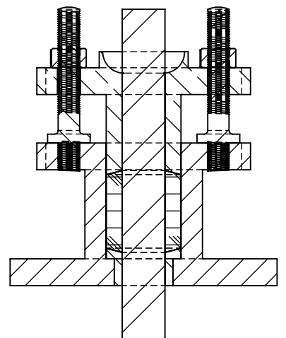
SECTION C-C SCALE 1 : 3
