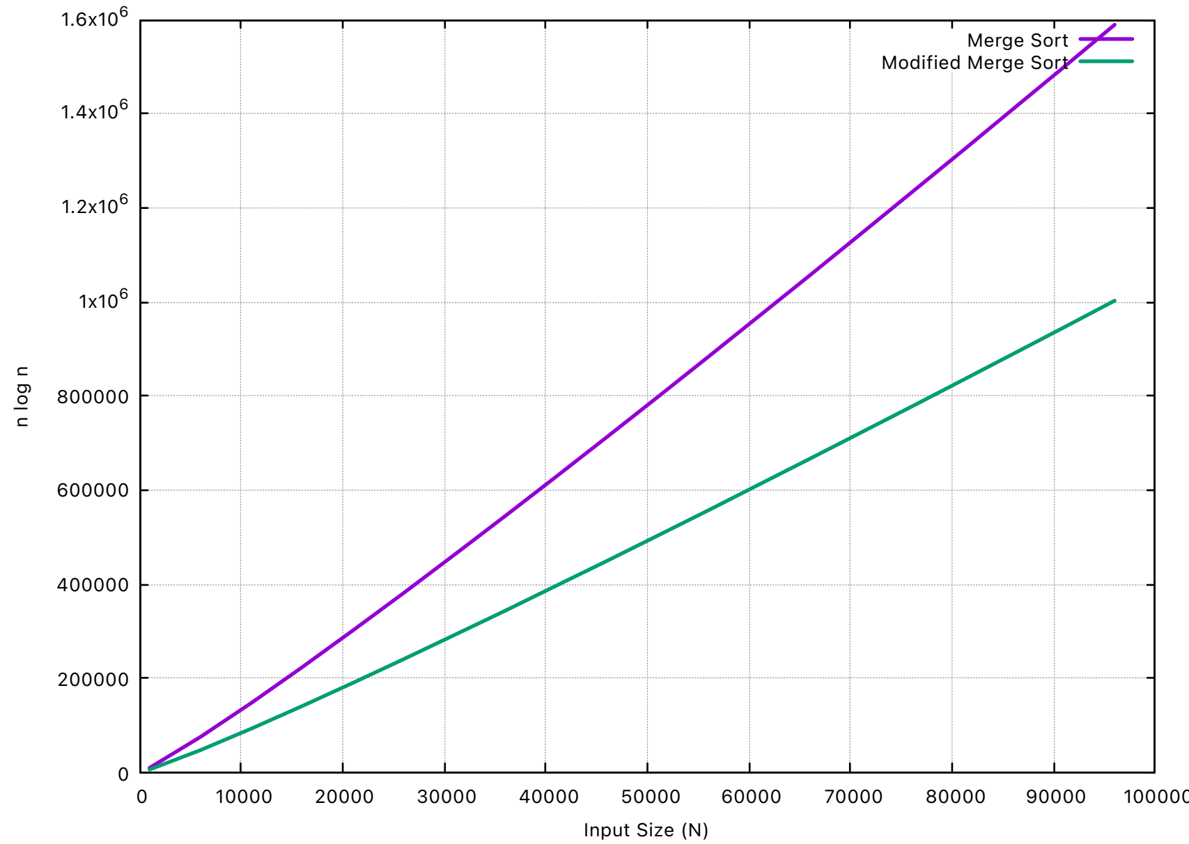
Merge Sort vs Modified Merge Sort
