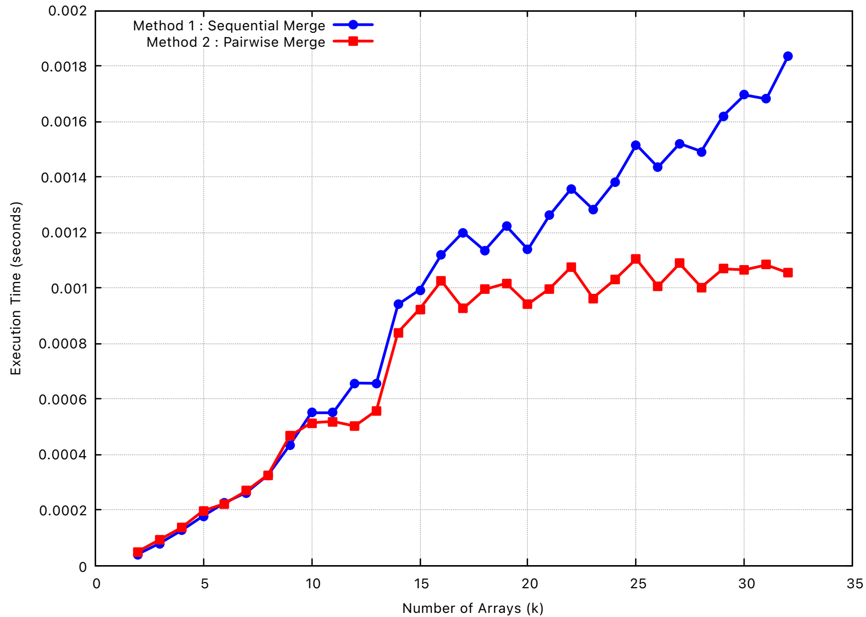
Comparison of Merging k Sorted Arrays
