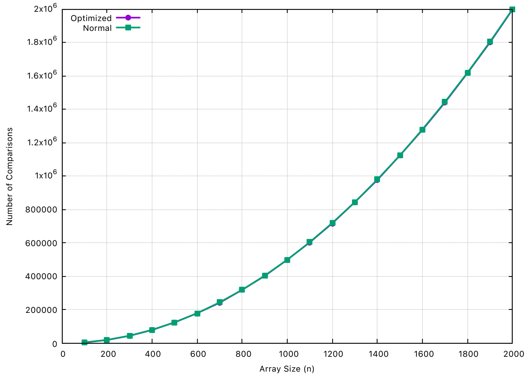
Bubble Sort Performance Analysis
