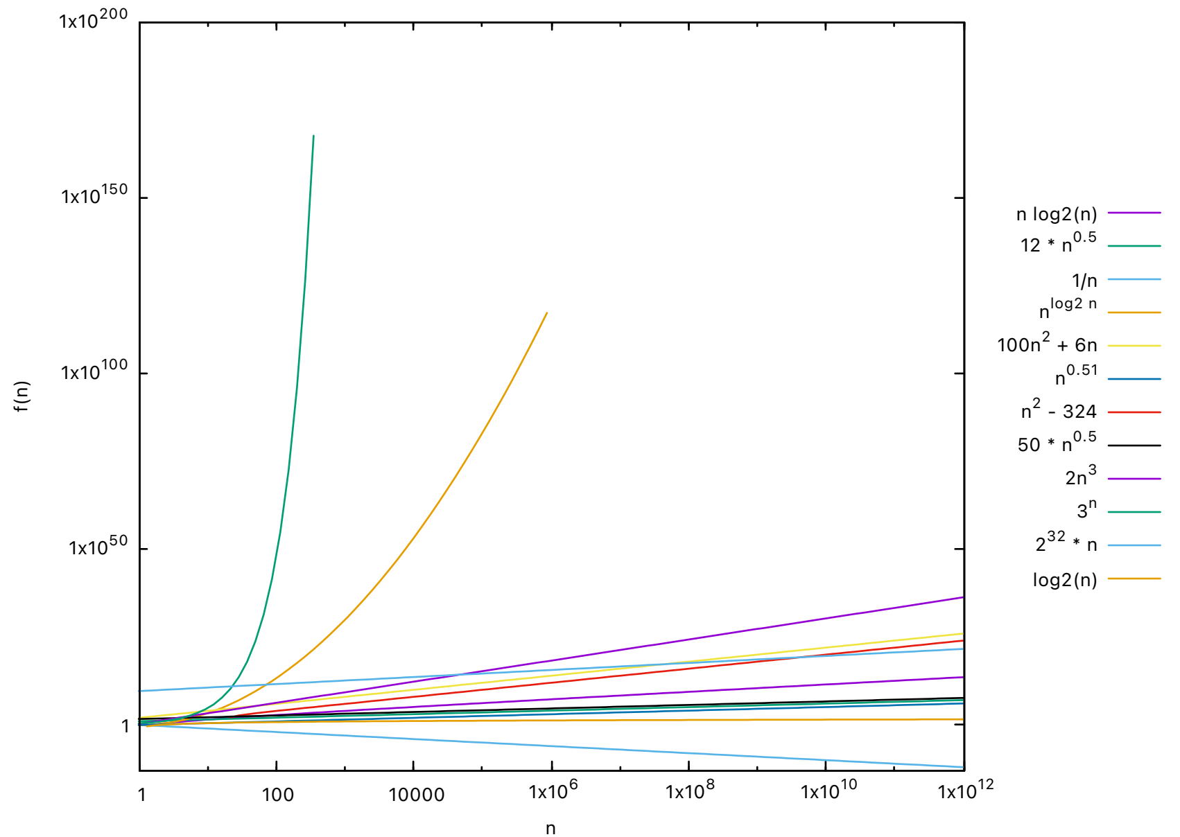
Asymptotic Growth Rates of Functions
