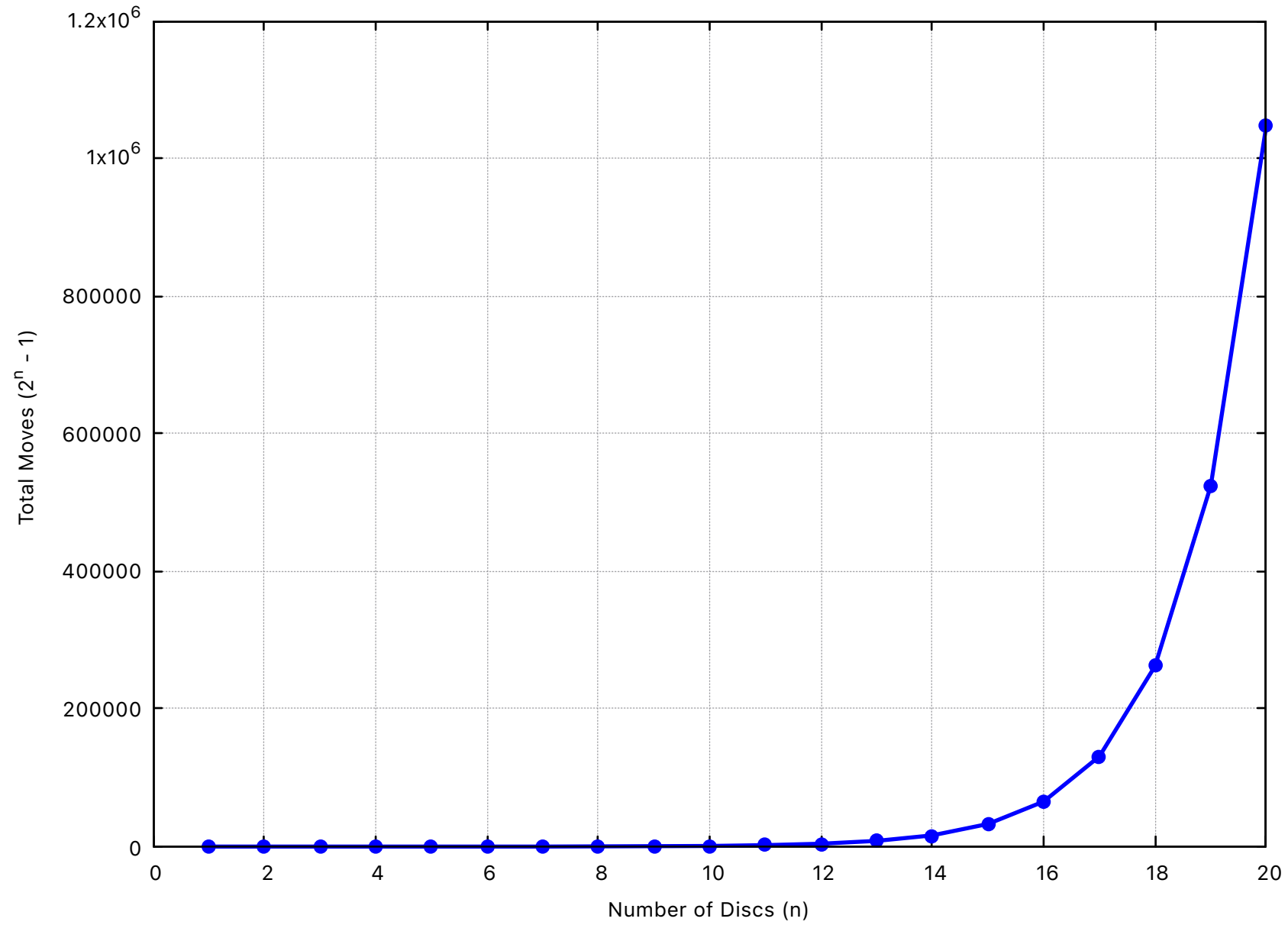
Tower of Hanoi Analysis
