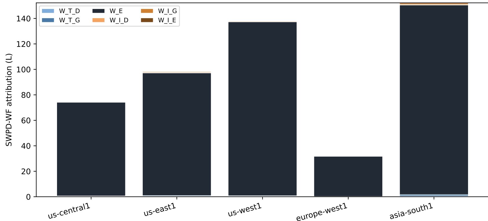
Per-region SWPD-WF attribution vector (phase × flow)
