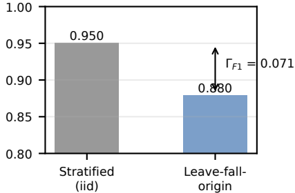
Transfer gap (mean F1)
