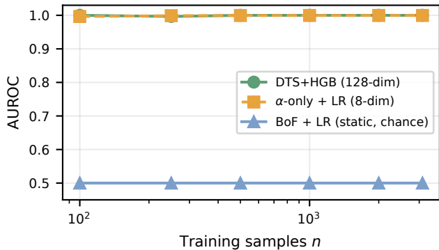
Controlled temporal-order benchmark
