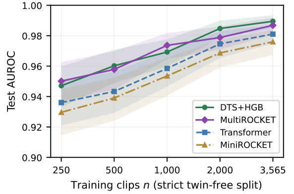
Figure 1: Sample efficiency on the strict twin-free split: test AUROC versus training-set size for DTS+HGB, the strongest learned baselines (Transformer, MiniROCKET), and MultiROCKET (transform refit per subsample; shaded bands are 95% bootstrap intervals; validation and test sets fixed). DTS+HGB dominates the Transformer and MiniROCKET at every size and tracks MultiROCKET within overlapping intervals.
