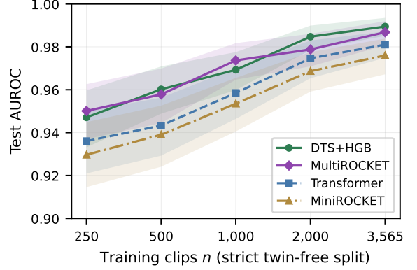
Figure 1: Sample efficiency on the strict twin-free split: test AUROC versus training-set size for DTS+HGB, the strongest originally evaluated baselines (Transformer, MiniROCKET), and the added MultiROCKET (transform refit per subsample; shaded bands are 95% bootstrap intervals; validation and test sets fixed). DTS+HGB dominates the originally evaluated baselines at every size and trades the lead with MultiROCKET within overlapping intervals.
