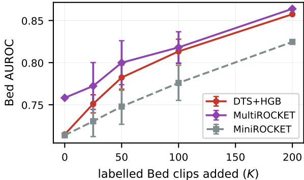
Few-shot Bed recovery (matched protocol)
