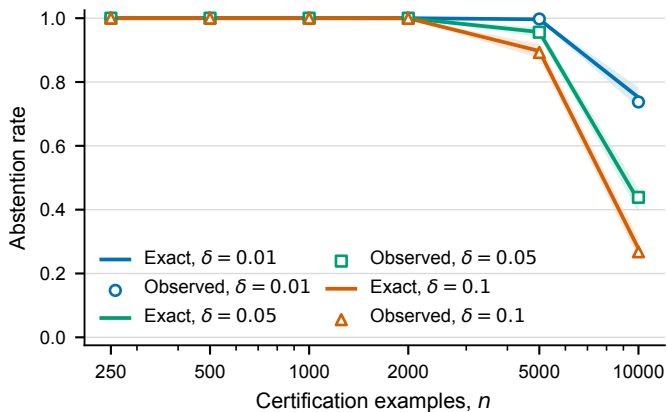
c Abstention at \Gamma = 1.25
