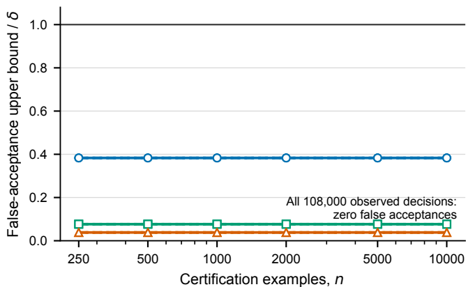
d Simultaneous safety bound
