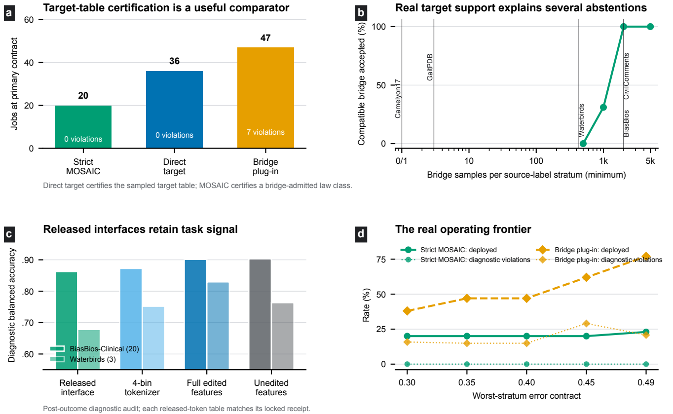
Figure 1: Additional audited evidence. (a) The direct target-table rule releases 36/100 jobs; strict MOSAIC releases 20/100 under the bridge-admitted population class. (b) Real bridge stratum support is overlaid on the locked bridge-power curve. (c) The released interfaces retain task signal on untouched diagnostics. (d) Deployment and observed diagnostic-violation rates across the registered utility frontier.
