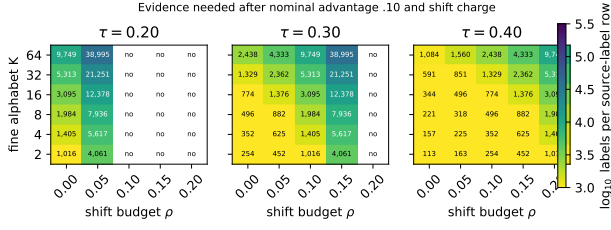
Figure 3: Sufficient labels per source-label stratum as a function of alphabet size, source contract, and charged shift budget. Blank cells are population-infeasible before sampling. The machine-readable chart contains all 120 registered configurations.
