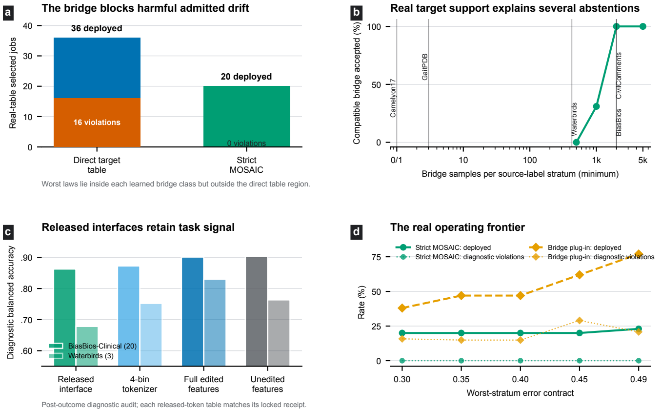
Figure 1: Additional audited evidence. (a) In a post-hoc stress test under real-table-anchored laws in the learned bridge class, the direct rule violates 16/36 accepted contracts; MOSAIC releases 20 safely and abstains on those 16 cases. (b) Real bridge stratum support is overlaid on the locked bridge-power curve. (c) The released interfaces retain task signal on untouched diagnostics. (d) Deployment and observed diagnostic-violation rates across the registered utility frontier.
