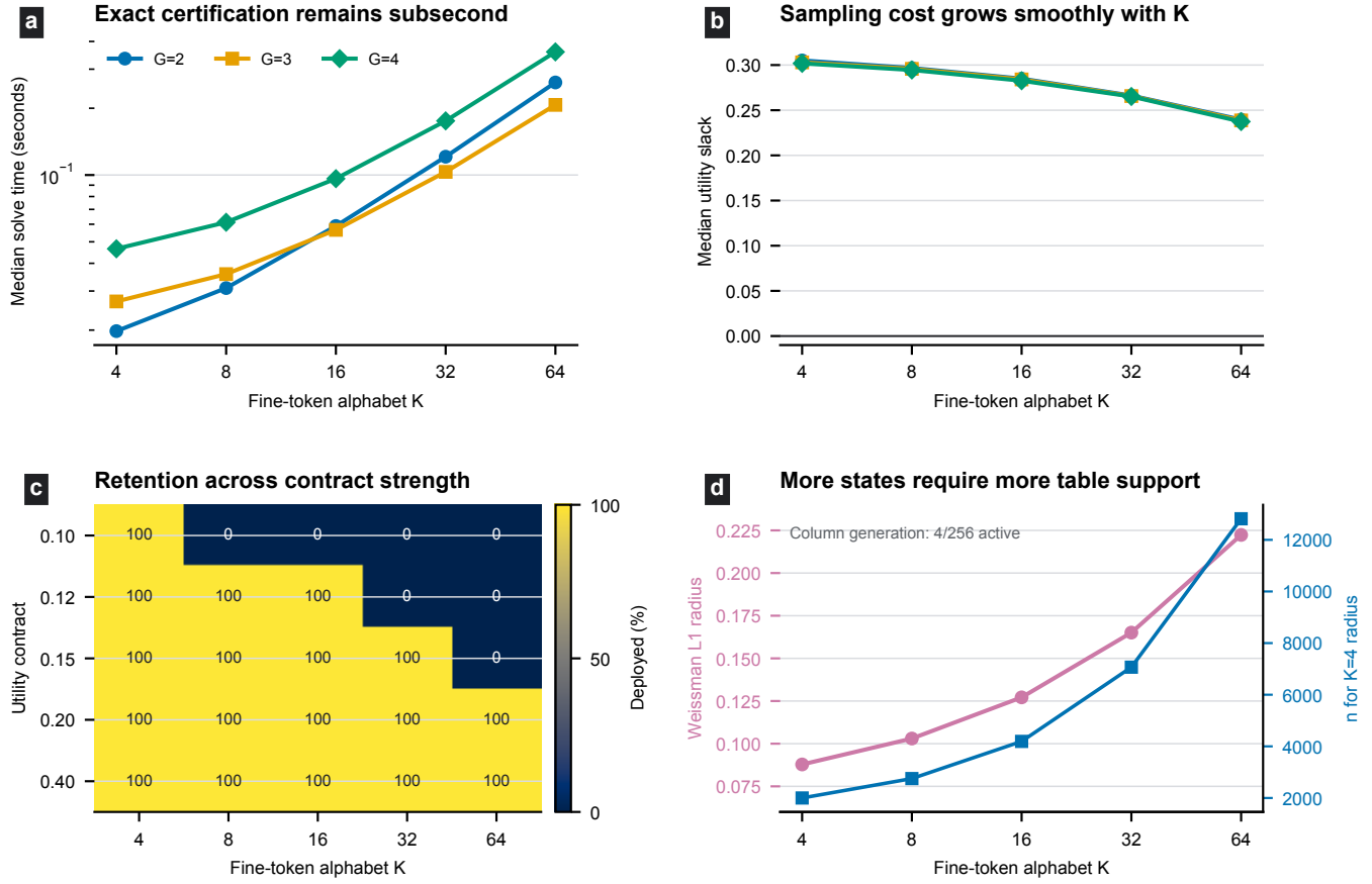
Figure 2: Finite-alphabet scaling over five independent tables per cell. (a) Median wall-clock optimization. (b) Median utility slack at the .40 contract. (c) Retention averaged over G = 2, 3, 4 at tighter contracts. (d) The Weissman radius and per-stratum sample size needed to recover the K = 4 radius for G = 4 . A G = L = 4 constraint-generation stress uses 4 of 256 possible attacker assignments.
