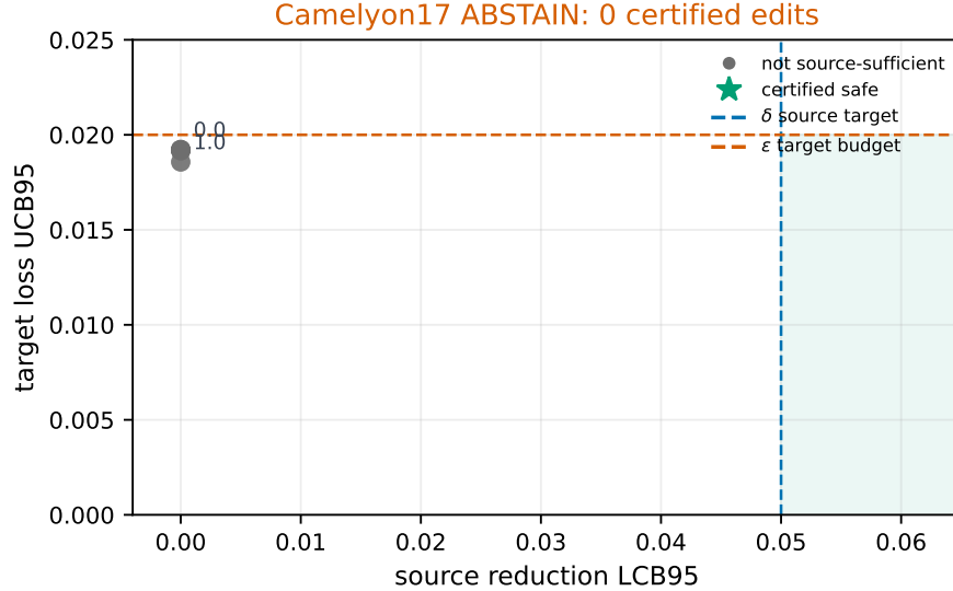
Figure 3: Full Camelyon17 projection frontier certificate. The green feasible region requires both source-reduction and target-preservation bounds. No candidate enters the feasible region, so VERA returns ABSTAIN.
