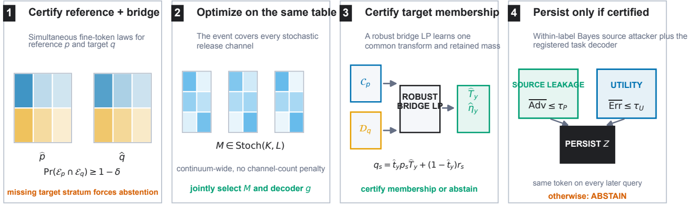
Figure 1: MOSAIC jointly certifies reference and labeled target-bridge token laws, optimizes a continuum of source-blind stochastic channels on that event, and uses a robust bridge LP to certify target membership. The runtime samples one persistent token only when within-label source distinguishability and registered task utility pass; otherwise it abstains. The primary contract is within-label source distinguishability.
