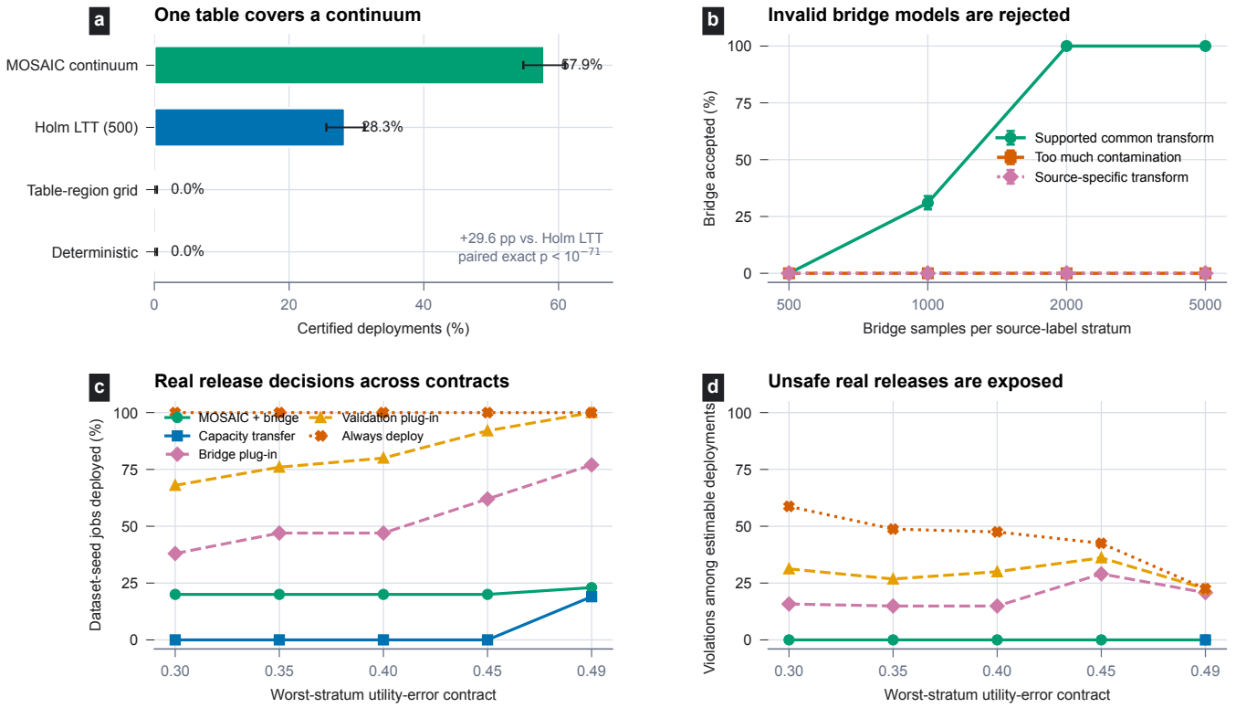
Figure 3: Audited evidence beyond the primary synthetic comparison. (a) One table-wide event certifies 57.9% of low-data trials versus 28.3% for Holm LTT over 500 matched candidates. (b) Bridge evidence gains power for a valid common transform while rejecting two registered violations. (c) Across 100 real dataset-seed jobs, strict MOSAIC deploys 20% through the .45 utility contract and 23% at .49. (d) It records no external diagnostic violation; plug-in rules violate 14.9–36.1% of their estimable deployments. Validation-only and unconditional rules additionally deploy all 20 unestimable Camelyon jobs.
