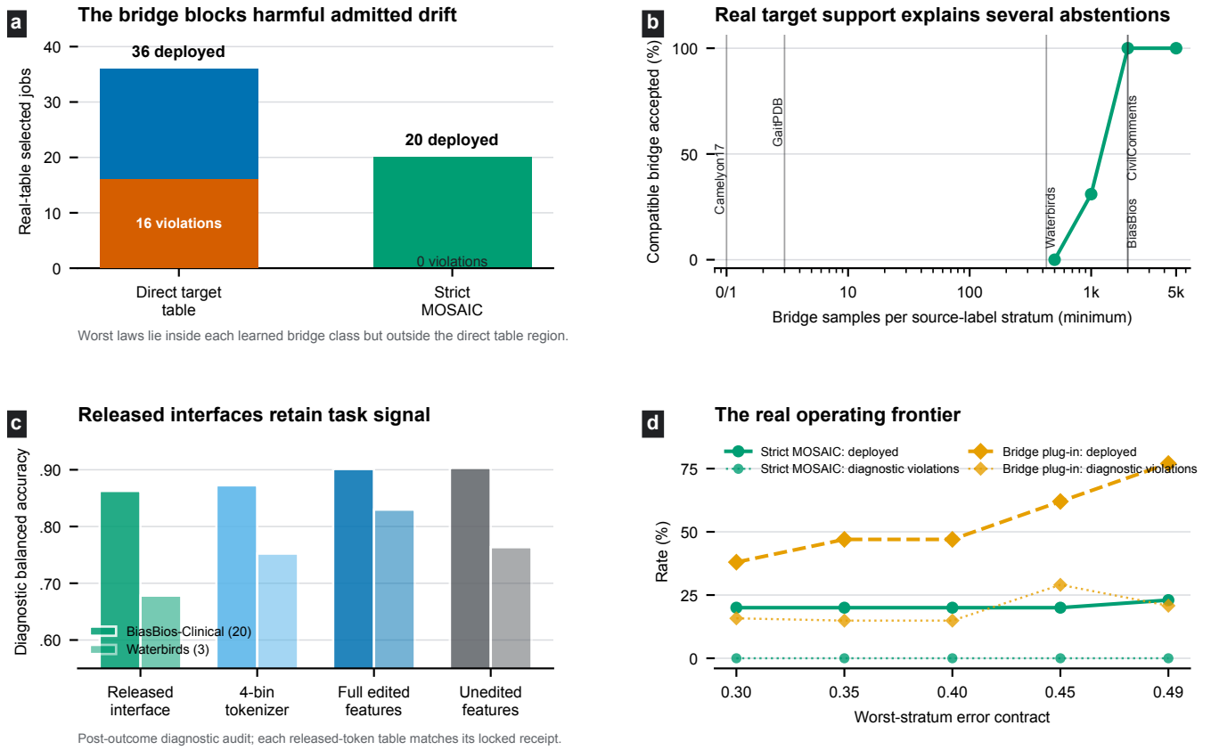
Figure 1: Additional audited evidence. (a) Under real-table-anchored laws in the learned bridge class, the direct rule violates 16/36 accepted contracts; MOSAIC releases 20 safely and abstains on those 16 cases. (b) Real bridge stratum support is overlaid on the locked bridge-power curve. (c) The released interfaces retain task signal on untouched diagnostics. (d) Deployment and observed diagnostic-violation rates across the registered utility frontier.
