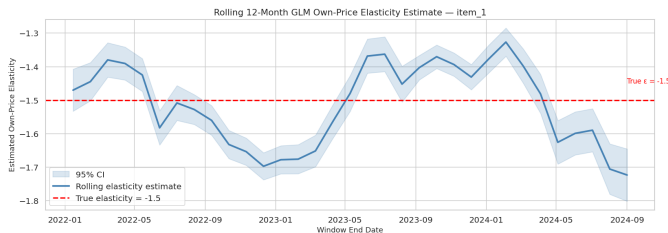
Fig. 7: Rolling twelve-month GLM own-price elasticity for Item 1 (30-day step). Blue line: point estimate; shaded band: approximate 95% interval; red dashed: simulator truth ( \epsilon = -1.50 ).
