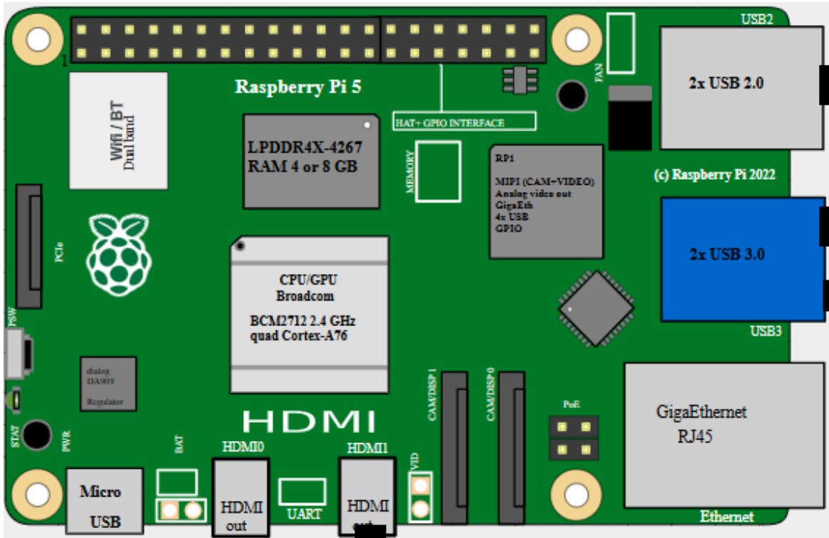
Raspberry Pi 5
