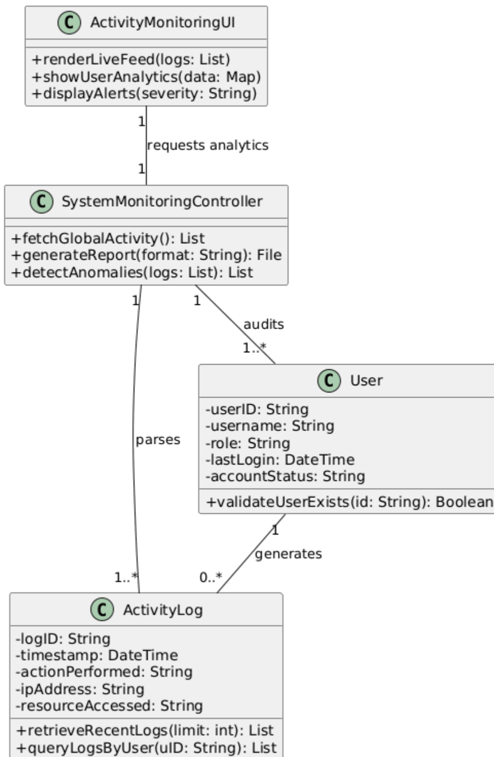
Class Diagram: Monitor System Activity (Detailed)
