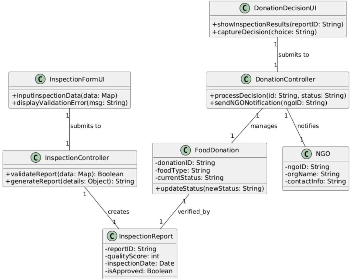
Class Diagram: Accept/Reject Food Donation (Detailed)
