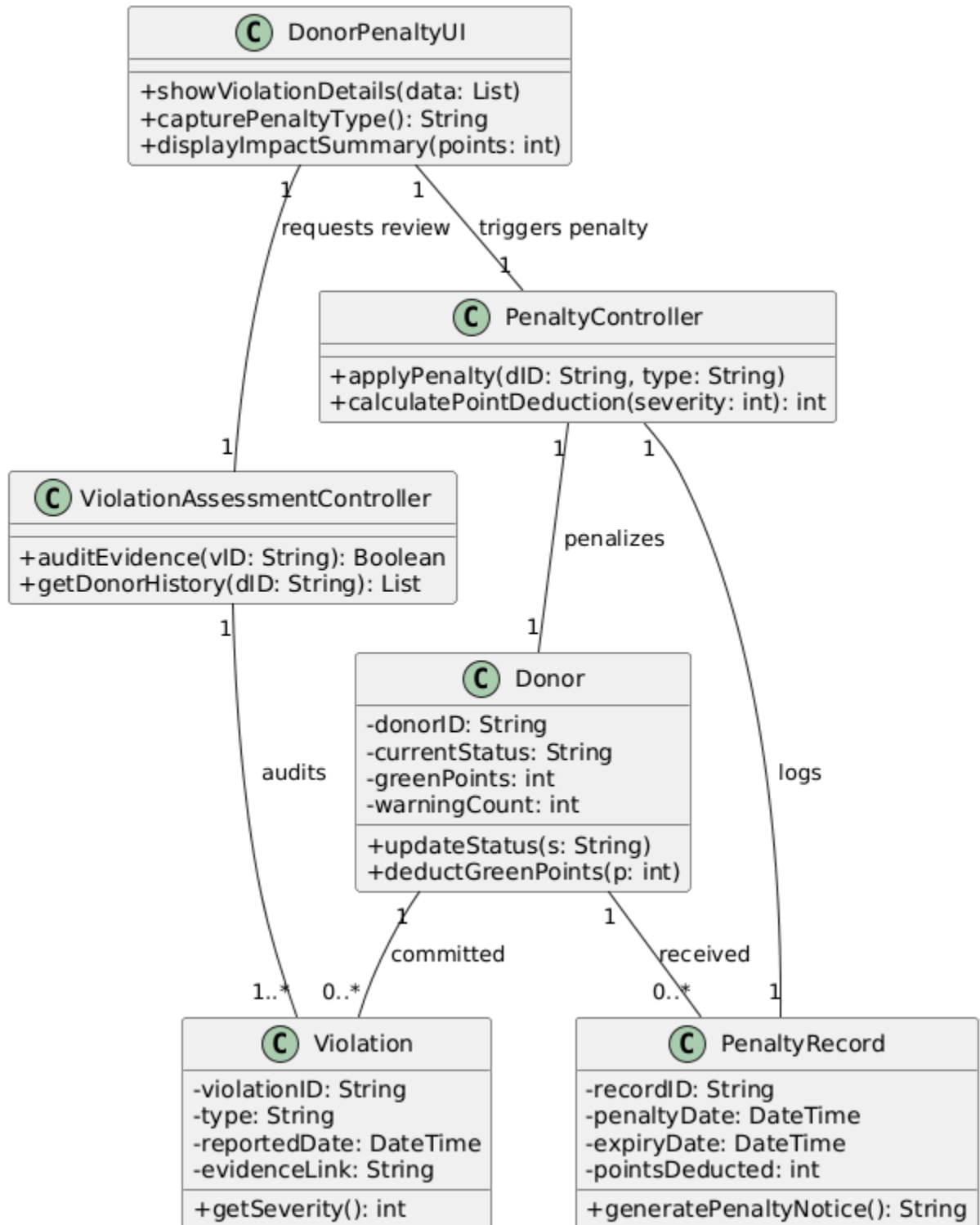
Class Diagram: Penalize Food Donor (Detailed)
