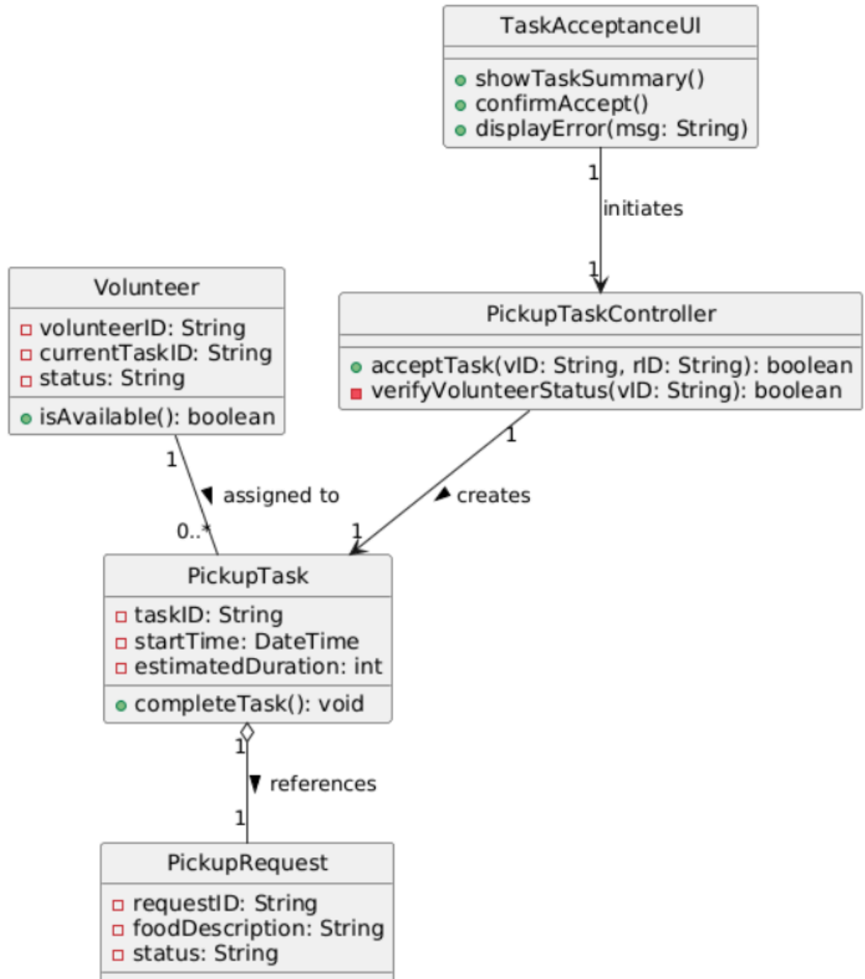
Class Diagram - Accept Pickup Task
