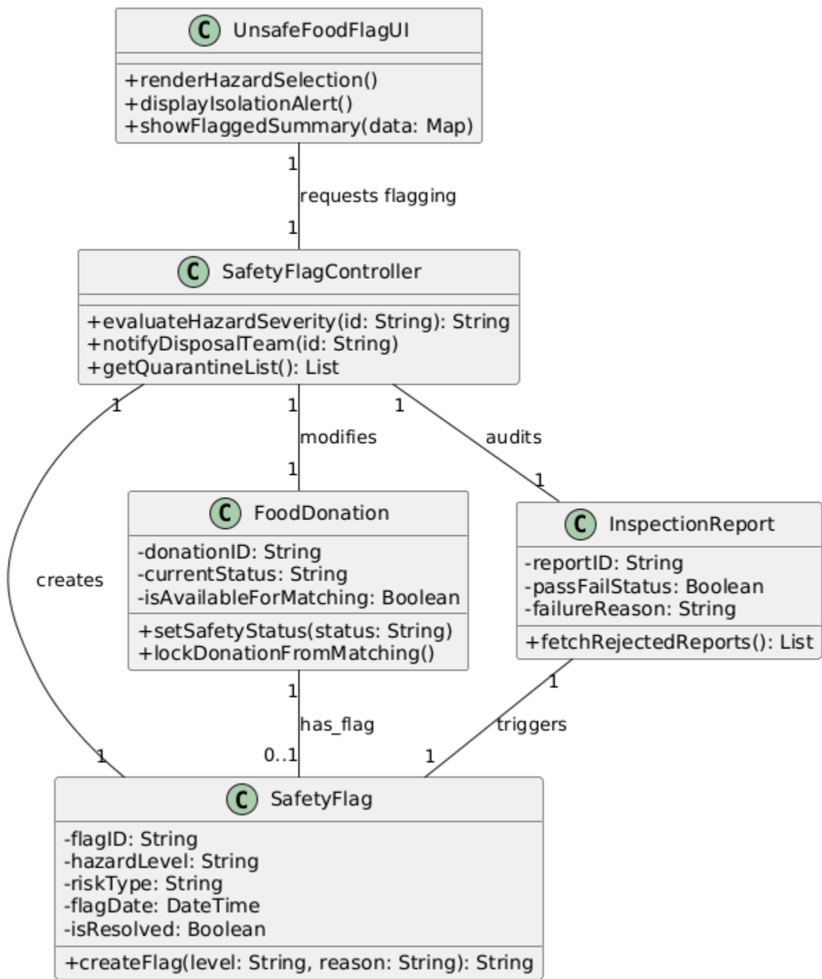
Class Diagram: Flag Unsafe Food (Detailed)
