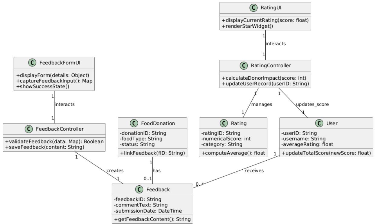
Class Diagram: Feedback & Rating System (Detailed)
