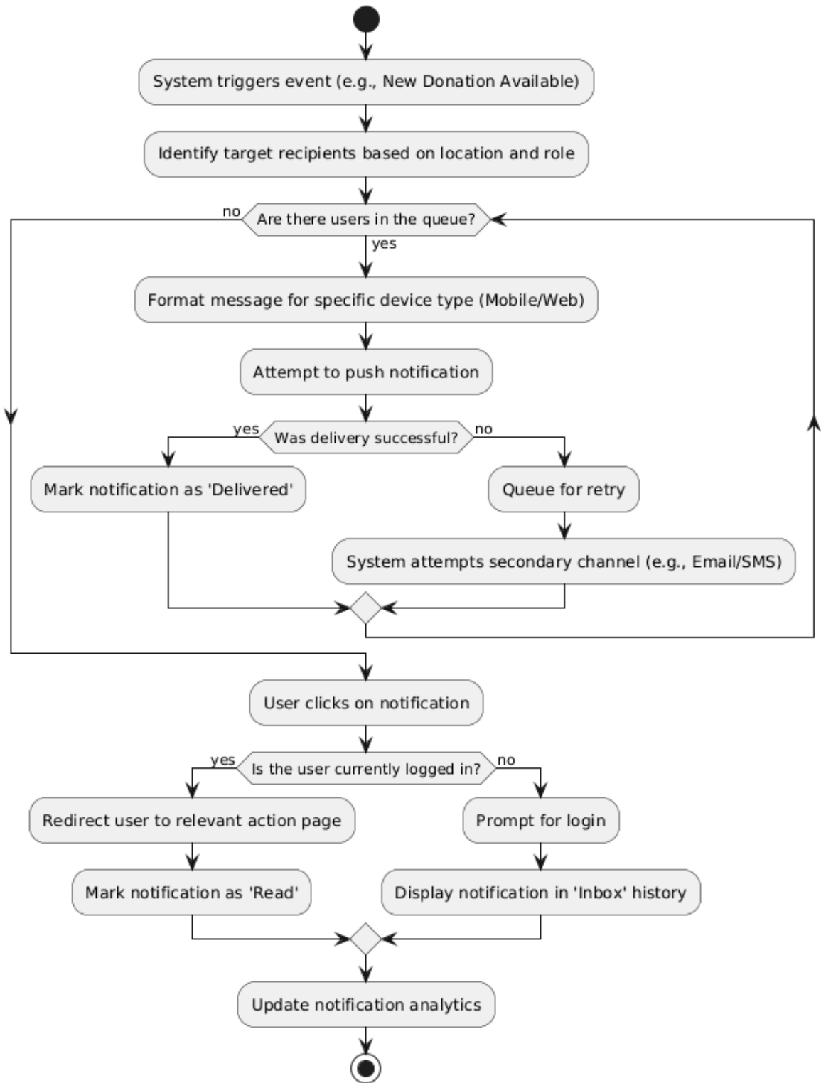
Activity Diagram - Real-Time Notification System (User Perspective)
