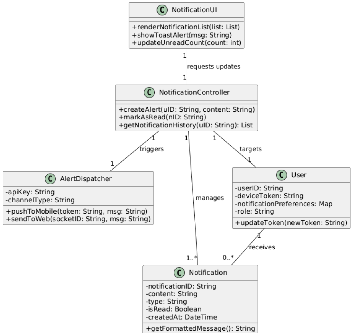
Class Diagram: Real-Time Notification System (Detailed)
