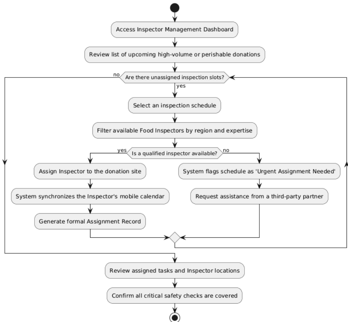
Activity Diagram - Assign / Manage Food Inspector (User Perspective)
