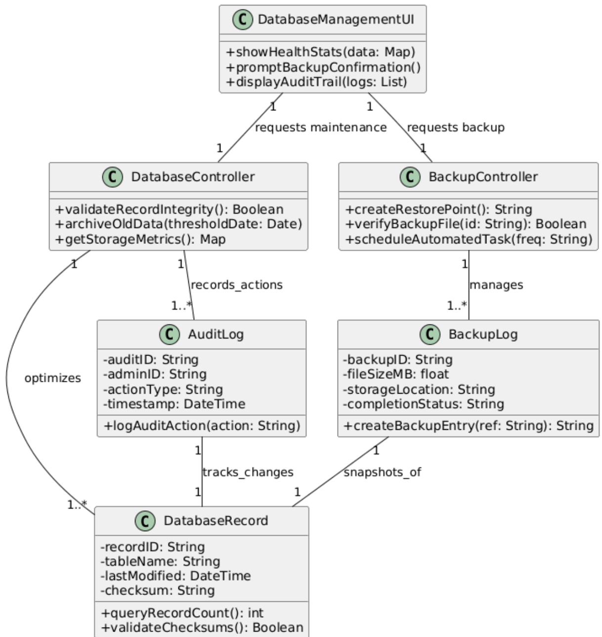
Class Diagram: Manage Records (Detailed)
