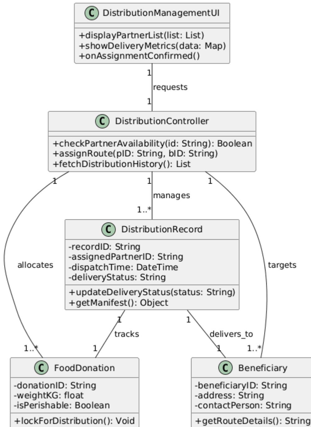
Class Diagram: Manage Delivery Partners (Detailed)
