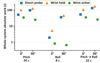
Fig. 5. Whole-system absolute joint mechanical work in 15 N contact simulations: pitch (0° → +30° → −30° → 0°, 24 s), roll (0° → 90°, 8 s), and their continuous sequence (32 s). The 0° and 90° groups retain distinct direct-probe baselines. Bars represent single runs; active totals include J8–J9. Results remain diagnostic: dynamics checks are unmet, with additional tracking violations in pitch and combined runs.
