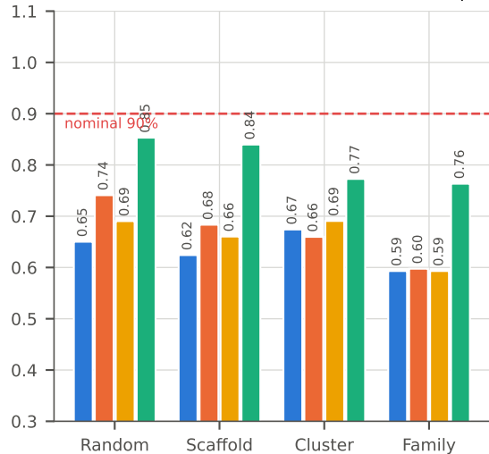
Marginal coverage: holds on random splits, fails under shift Least-familiar band: fails even on random splits
