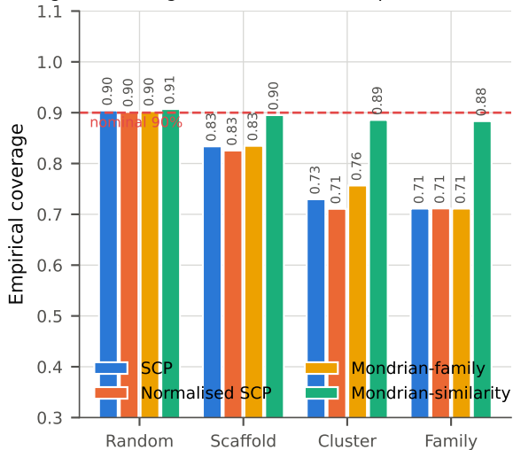
Marginal coverage: holds on random splits, fails under shift Least-familiar band: fails even on random splits
