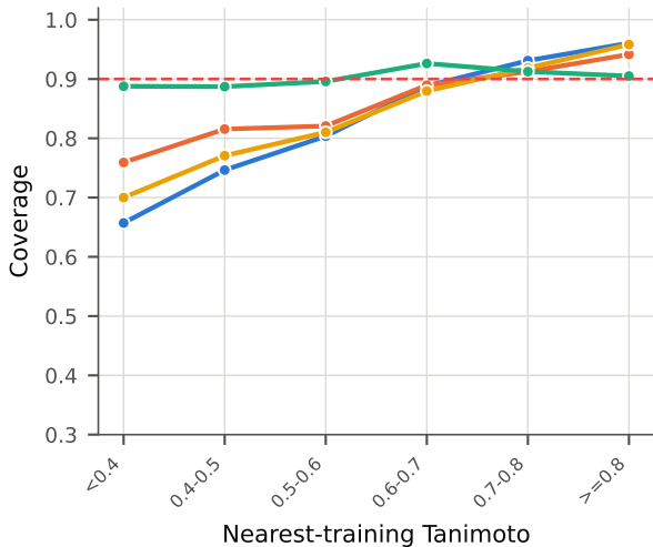
Random
