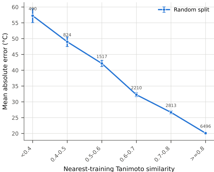
Error grows as the nearest training analogue recedes
