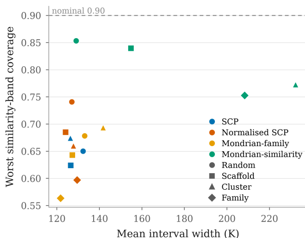
Figure 6. Split-averaged worst similarity-band coverage against mean interval width in K. Marker colour is the conformal method, shape the split regime. The coverage-width criterion is not plotted; it is reported in Table 7.
