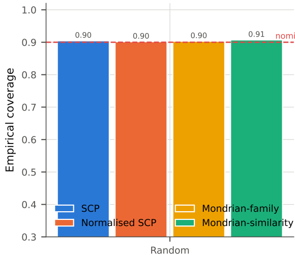
Marginal coverage looks fine everywhere
