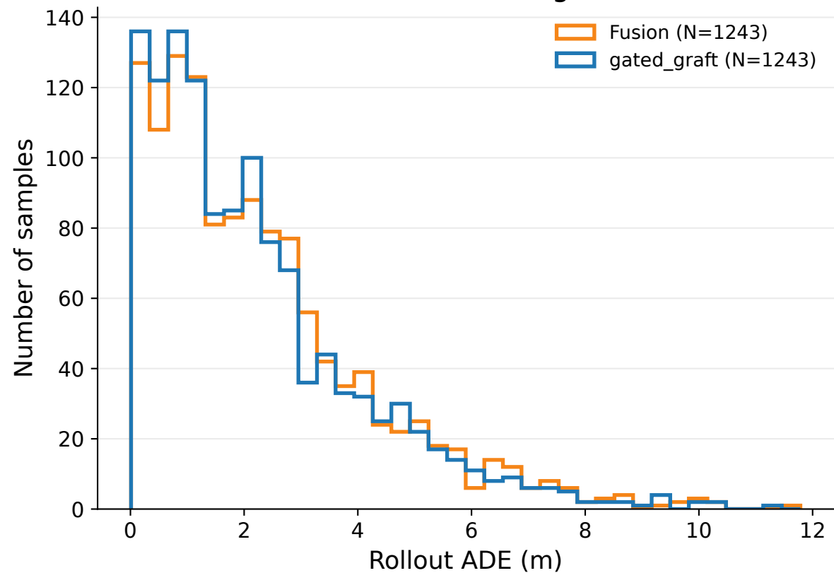
Rollout ADE Histogram
