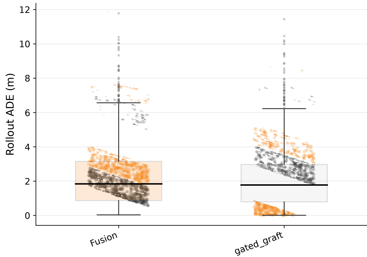
Rollout ADE Distribution
