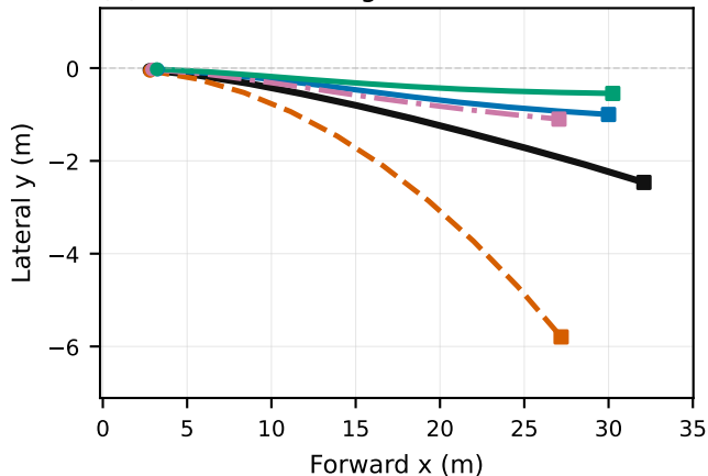
(c) Speed-changing
