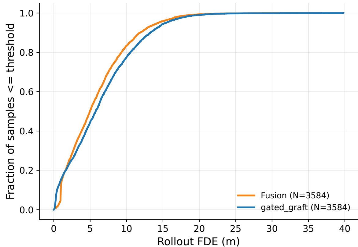
Rollout FDE ECDF
