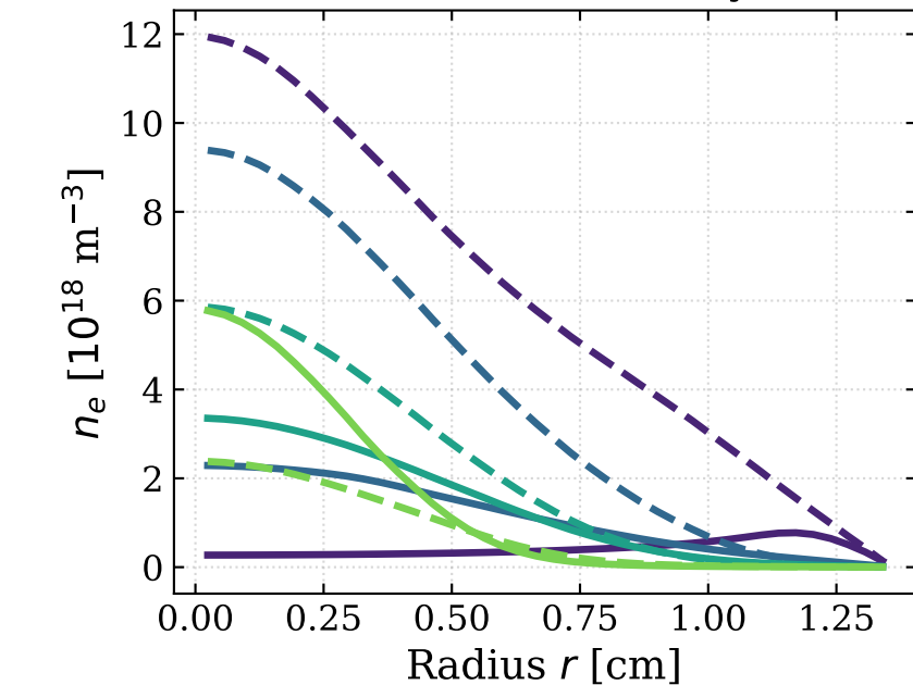
(e) Electron Density
