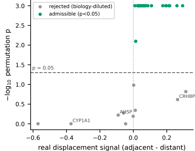
a Marker-validity null (1,000 perms) 28/38 admissible
