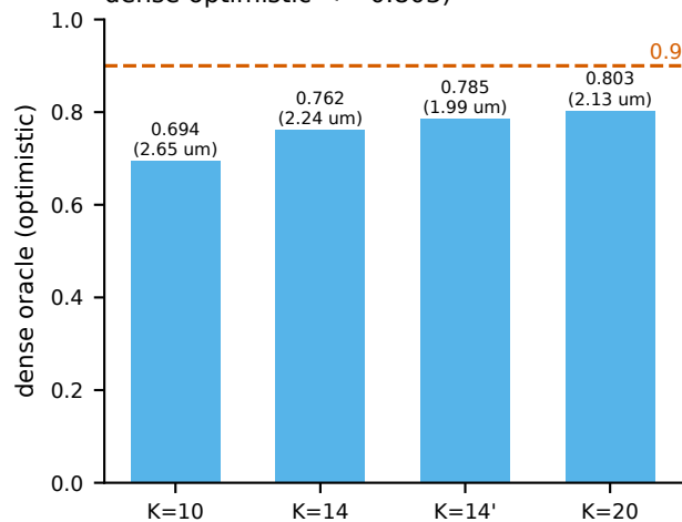
d Robustness: cell-typing (sigma 1.99-2.65, dense optimistic \leq 0.803 )
