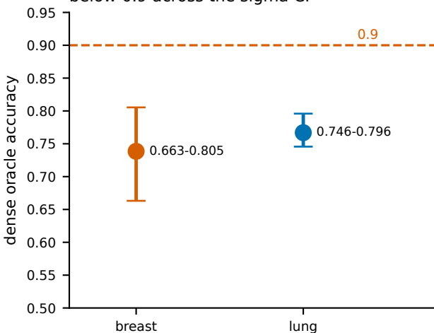
c Dense tissue ( \sim 13,600 cells/ \text{mm}^2 ) below 0.9 across the sigma CI
