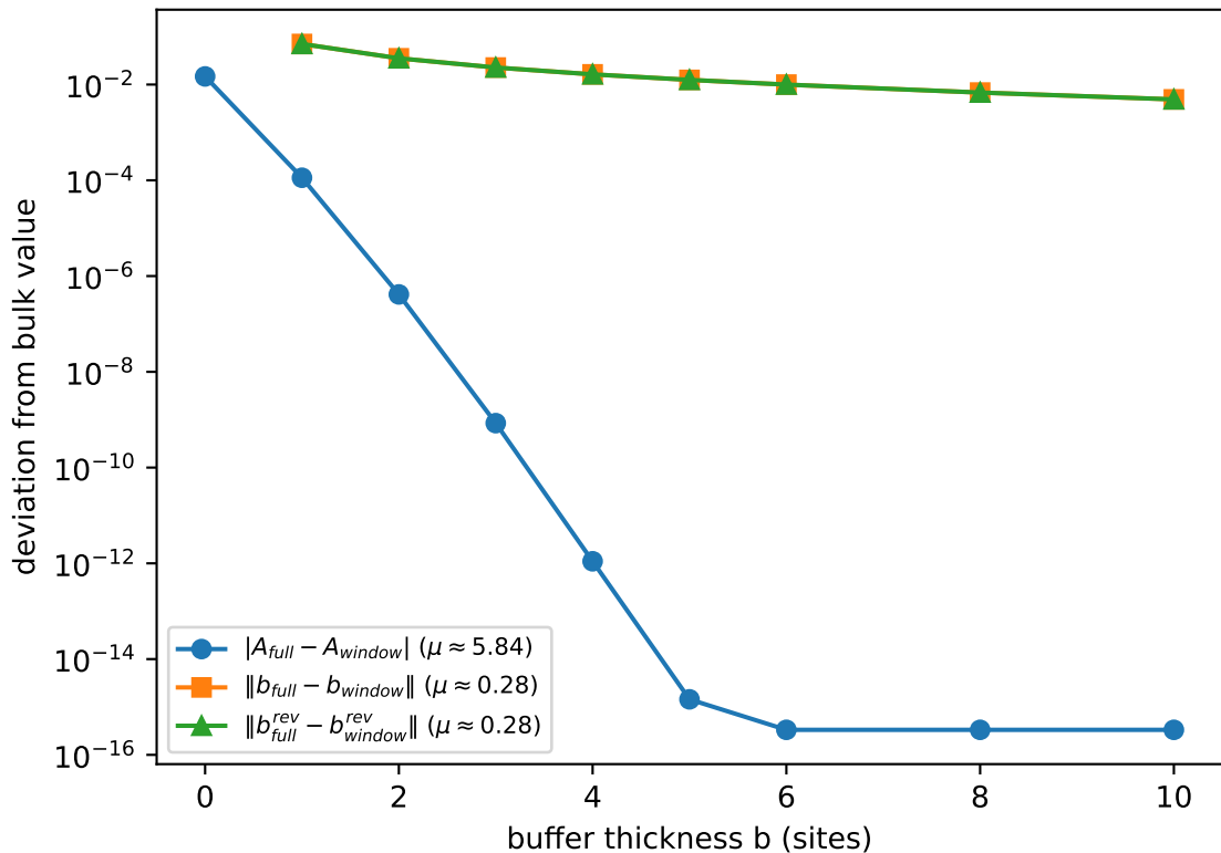
Buffered local-channel reduction (Plan A, free-fermion embedding)
