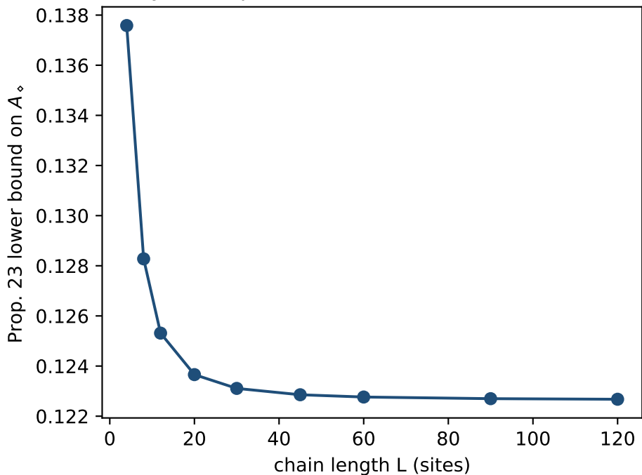
Thermodynamic persistence of the resource lower bound
