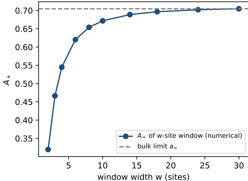
(a) windowed channel asymmetry converges
