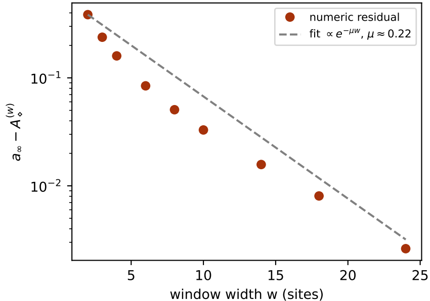
(b) exponential (quasi-local) convergence
