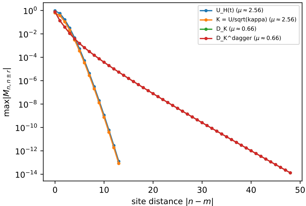
Lemma 1: quasi-locality of K , U , D_K
