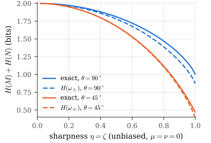
FIG. 5. Unsharp measurements ( \mu = \nu = 0 , \eta = \zeta ): exact minimum of H(M) + H(N) (solid) and the bound from Theorem 4 (dashed) for Bloch angles 90^\circ and 45^\circ .
