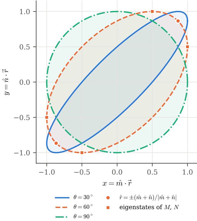
FIG. 1. The ellipse \mathcal{E}_\theta of achievable expectation values (x, y) = (\langle \hat{m} \cdot \vec{\sigma} \rangle, \langle \hat{n} \cdot \vec{\sigma} \rangle) for three Bloch angles. Markers (for \theta = 60^\circ ) show the two families of states that saturate the partial sums of \omega_\oplus : eigenstates of M or N (squares; k = 1, 3 ) and bisector states \hat{r} \propto \pm(\hat{m} + \hat{n}) (circles; k = 2 ). No single point saturates all partial sums (Proposition 1).
