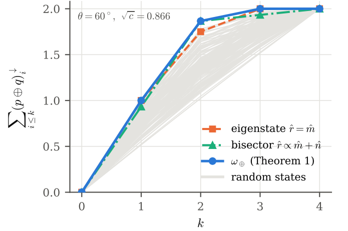
FIG. 2. Lorenz curves of p \oplus q for \theta = 60^\circ . Grey: 150 random states. The optimal bound \omega_\oplus (blue) is the upper envelope; it touches the eigenstate curve at k = 1, 3 and the bisector-state curve at k = 2 , but no single state reaches it.
