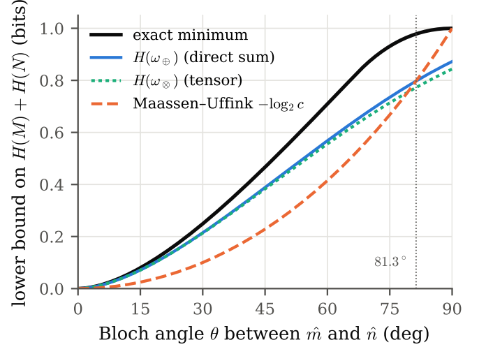
FIG. 3. Lower bounds on H(M) + H(N) as a function of the Bloch angle \theta ( c = \cos^2 \frac{\theta}{2} ). Black: exact minimum, equal to 2h(\frac{1+\sqrt{c}}{2}) for \theta \leq \bar{\theta} \approx 67.07^\circ . Blue: direct-sum bound h(\sqrt{c}) . Green (dotted): tensor-product bound h(w) . Orange (dashed): Maassen–Uffink. The direct-sum bound is stronger than MU for \theta < 81.3^\circ (dotted vertical line).
