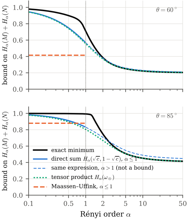
FIG. 4. Bounds on H_\alpha(M) + H_\alpha(N) across the Rényi family for \theta = 60^\circ (top) and \theta = 85^\circ (bottom). Black: exact minimum. Blue: direct-sum bound H_\alpha(\sqrt{c}, 1 - \sqrt{c}) of Corollary 1, valid for \alpha \leq 1 ; its thin dashed continuation for \alpha > 1 is not a bound and eventually exceeds the exact minimum. Green (dotted): tensor-product bound H_\alpha(\omega_\otimes) of Corollary 2. Orange (dashed): MU, valid for \alpha \leq 1 . The dotted vertical line marks the Shannon case \alpha = 1 .
