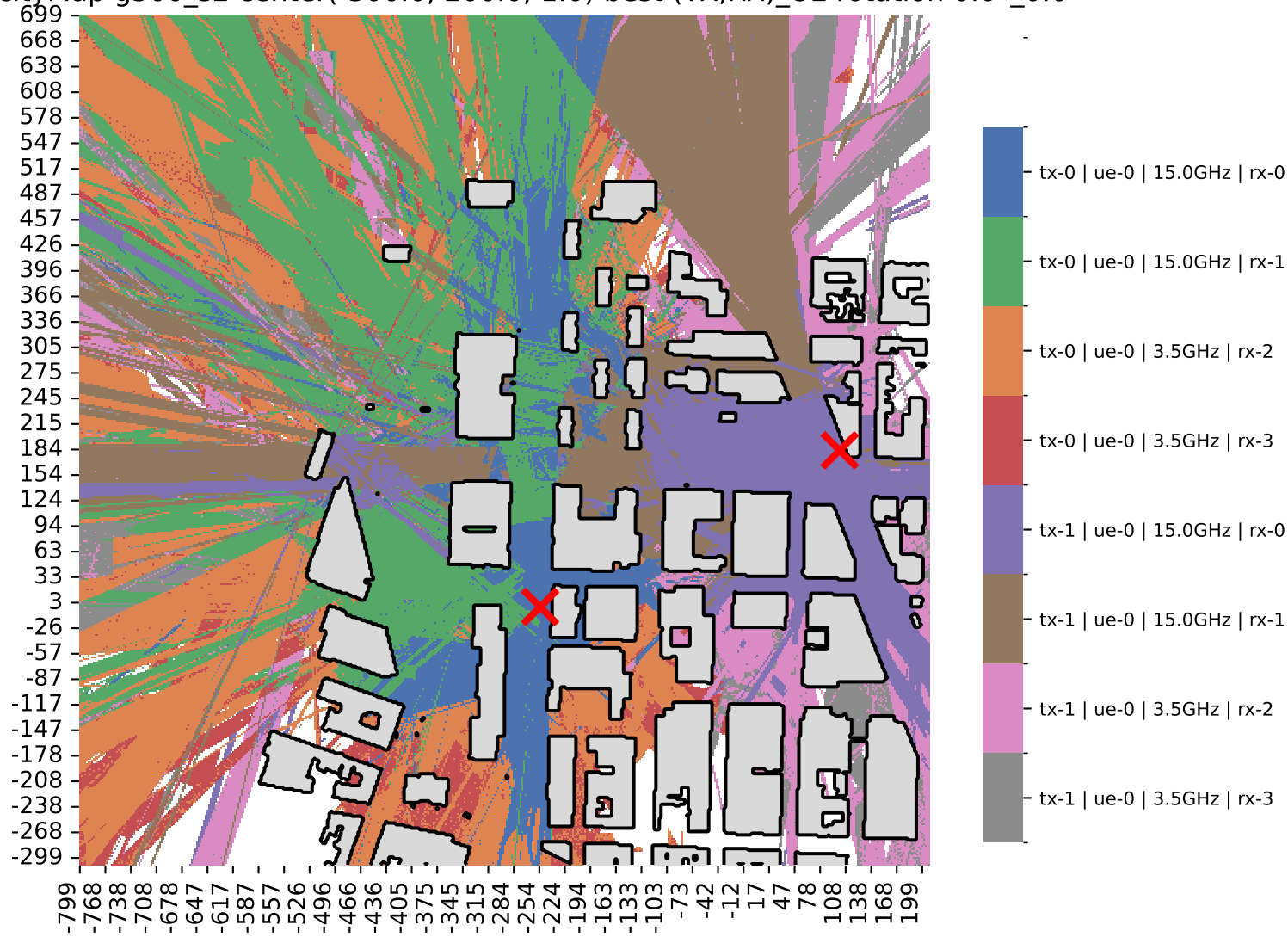
CapacityMap g500_s2 center(-300.0, 200.0, 1.0) best (TX,RX)_UE rotation 0.0°_0.0°
