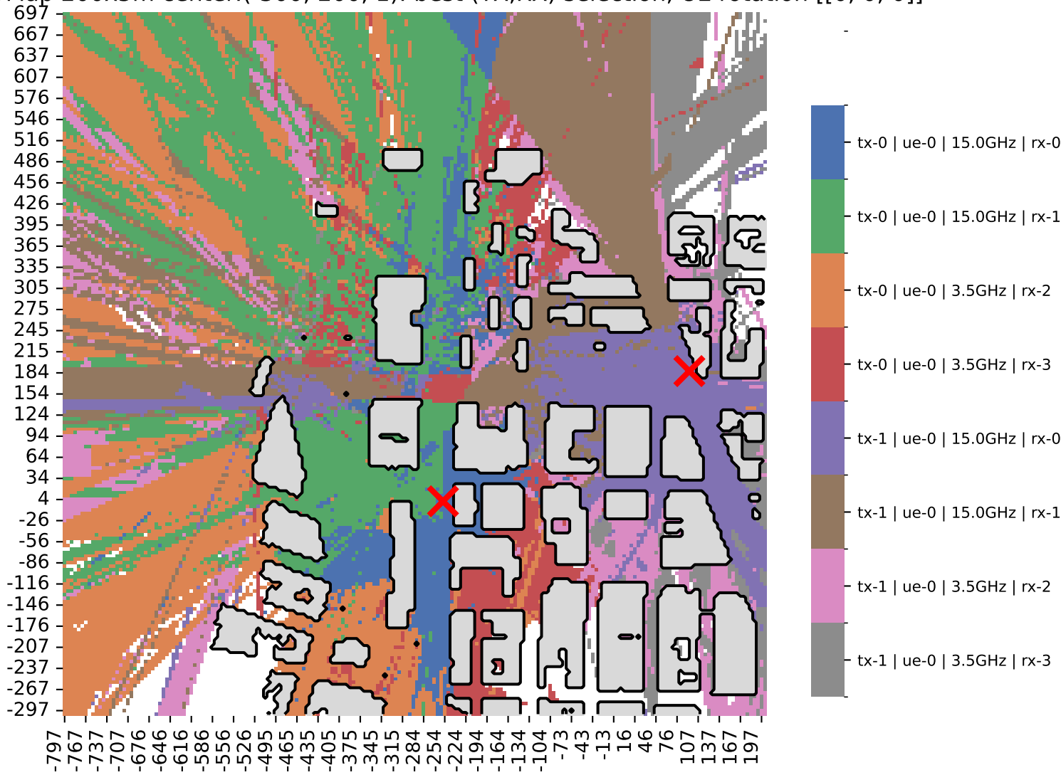
CapacityMap 200x5m center:(-300, 200, 1): best (TX,RX) selection, UE rotation [[0, 0, 0]]
