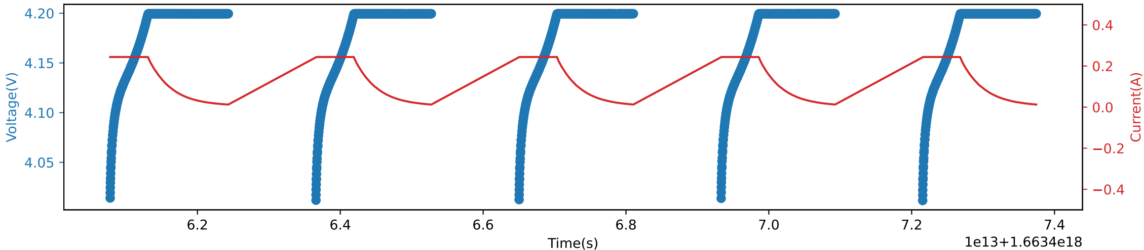
Voltage-Current vs time Profile
