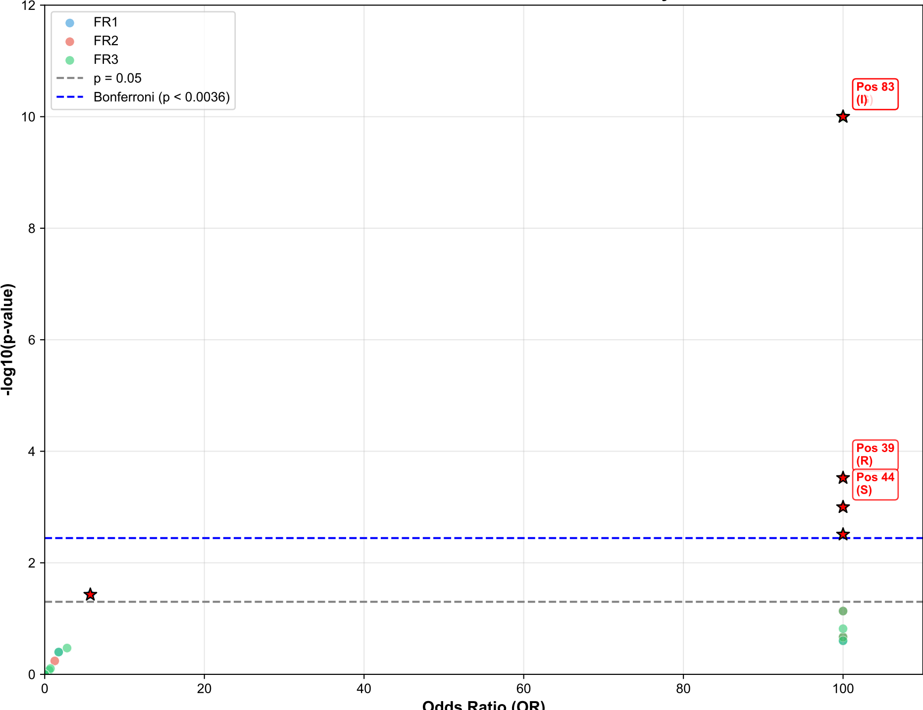
Volcano Plot: Fisher's Exact Test for VNAR Solubility Positions
