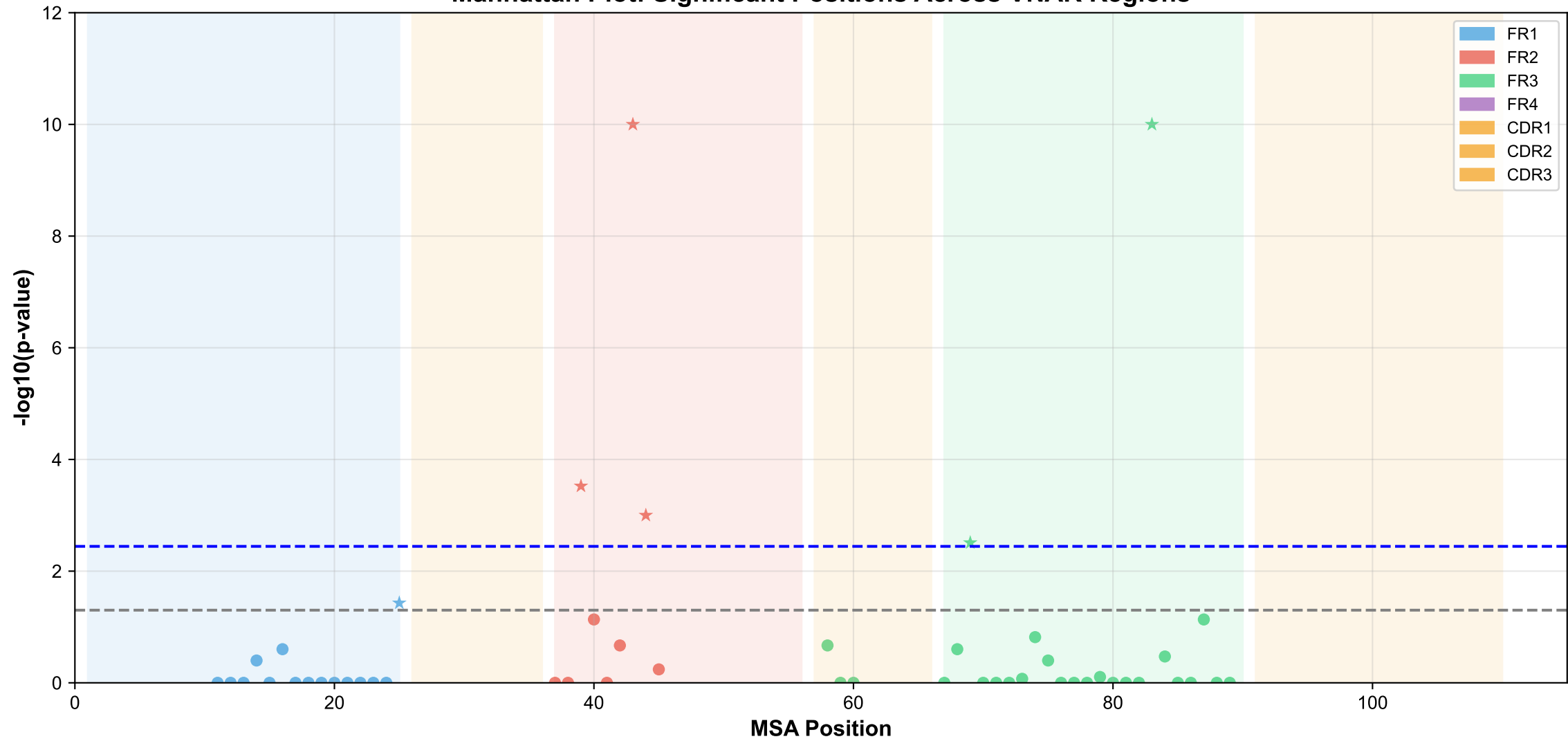
Manhattan Plot: Significant Positions Across VNAR Regions
