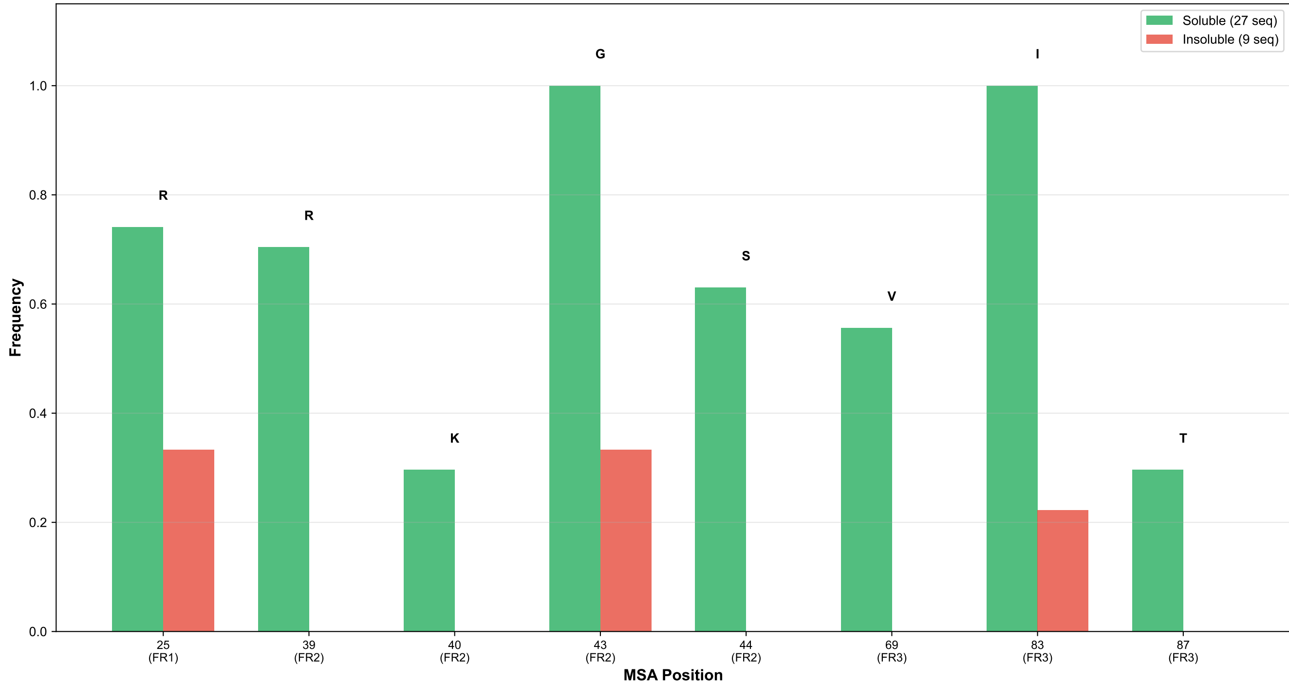
Amino Acid Frequency Comparison: Soluble vs Insoluble VNARs ( p < 0.1 positions)
