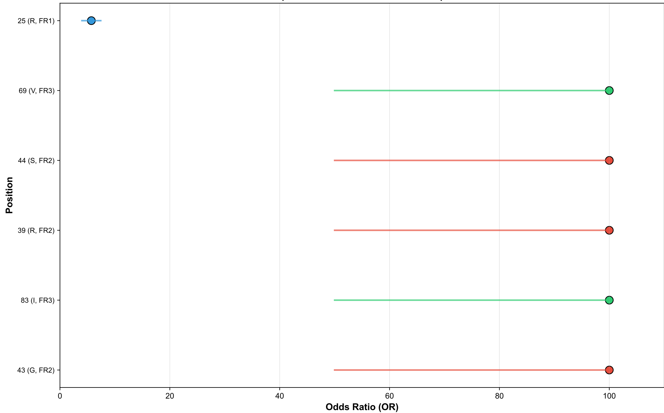
Forest Plot: Odds Ratio for Significant Positions (OR > 100 indicates infinite OR)
